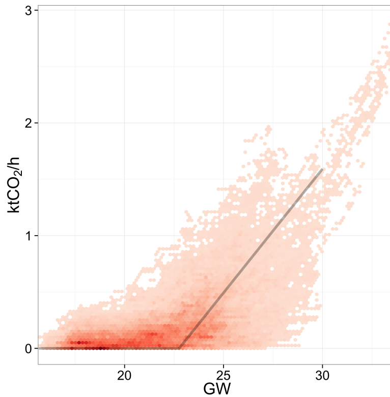
Figure 4.3: Emissions from thermal peaking plant (ktCO 2 -e per hour) vs system demand (total NEM generation). Use of peaking plant increases when system demand exceeds \sim 23 GW.
